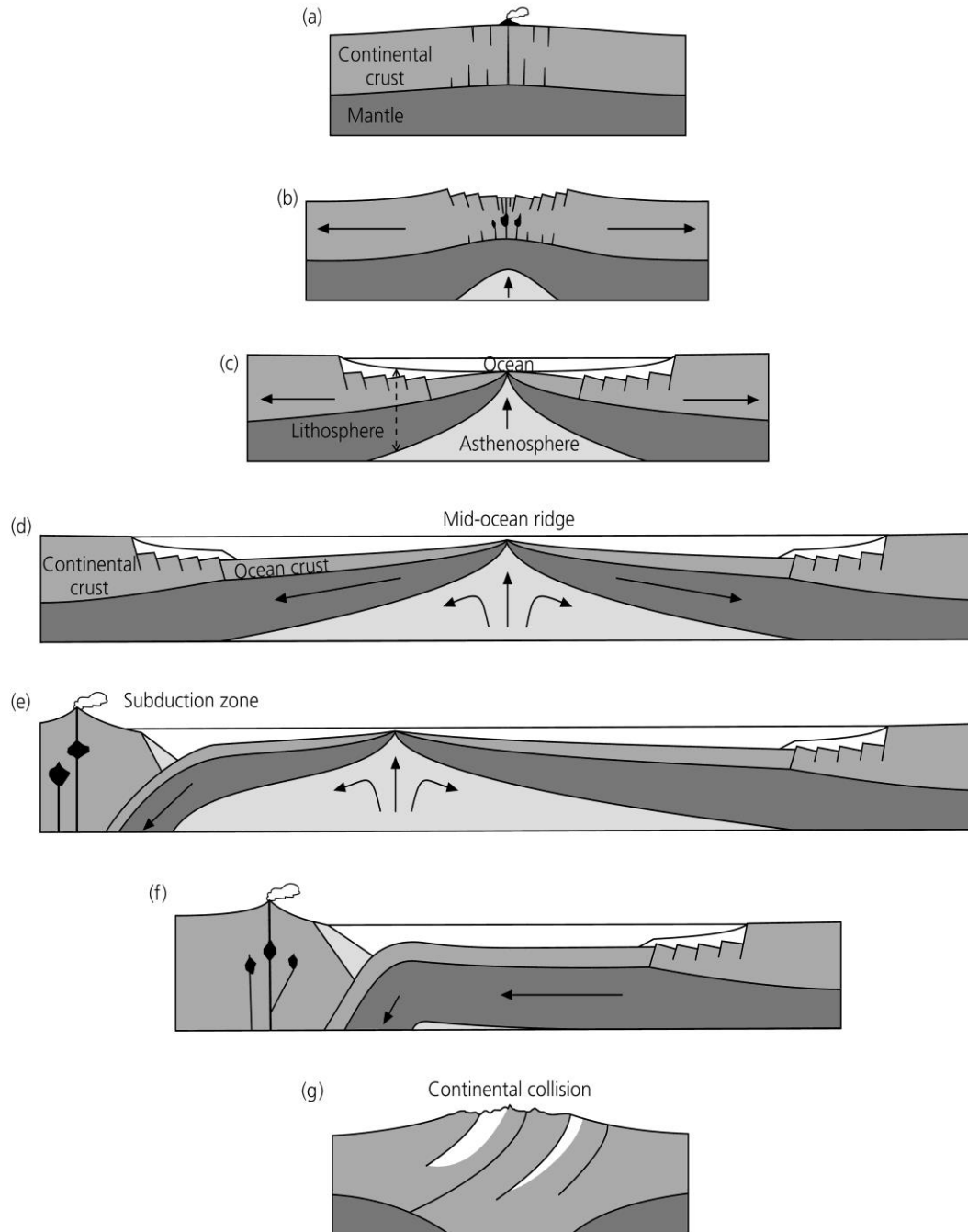
Figure 5.6-1: Schematic diagram of the Wilson cycle.
