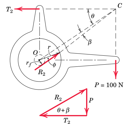
(b) Clockwise motion impends
