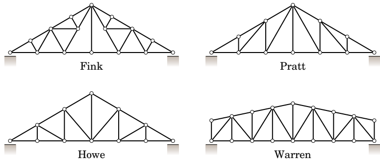
Commonly Used Roof Trusses
