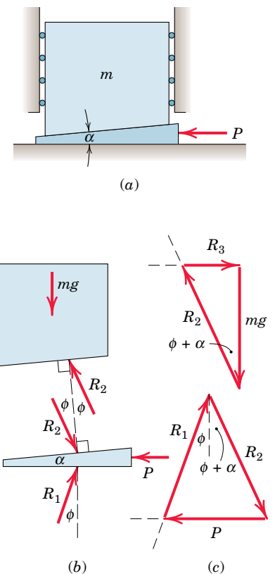
Forces to raise load
