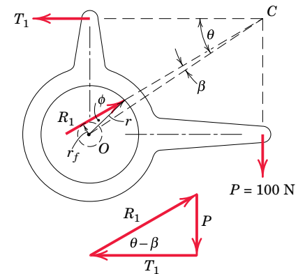
(a) Counterclockwise motion impends
