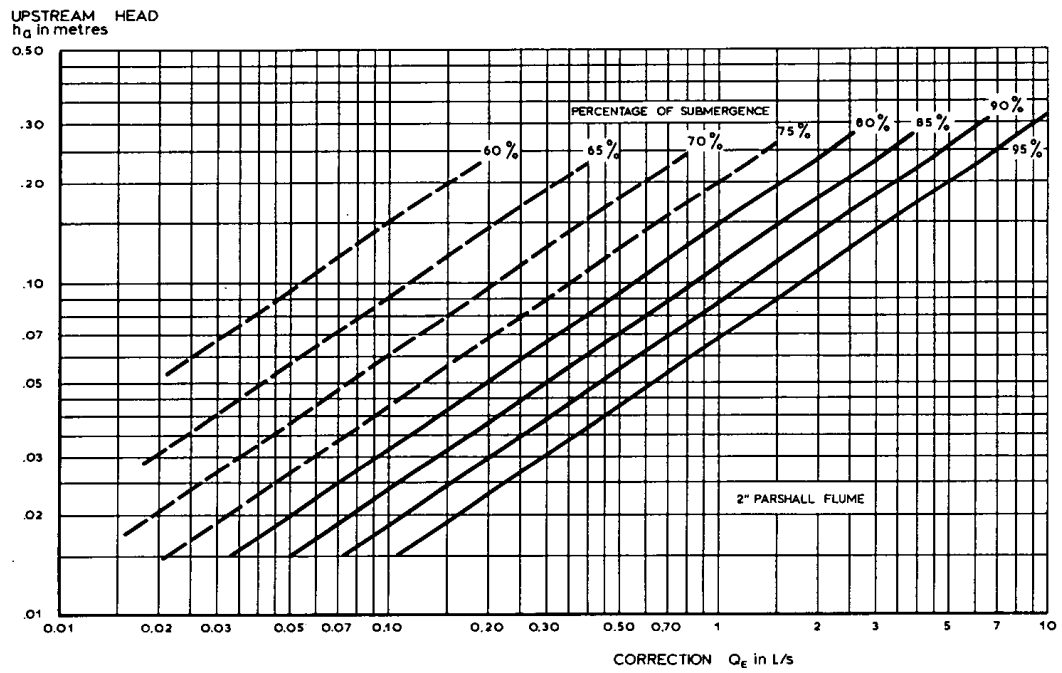
Figure 7.11 Discharge correction for submerged flow; 2" Parshall flume
