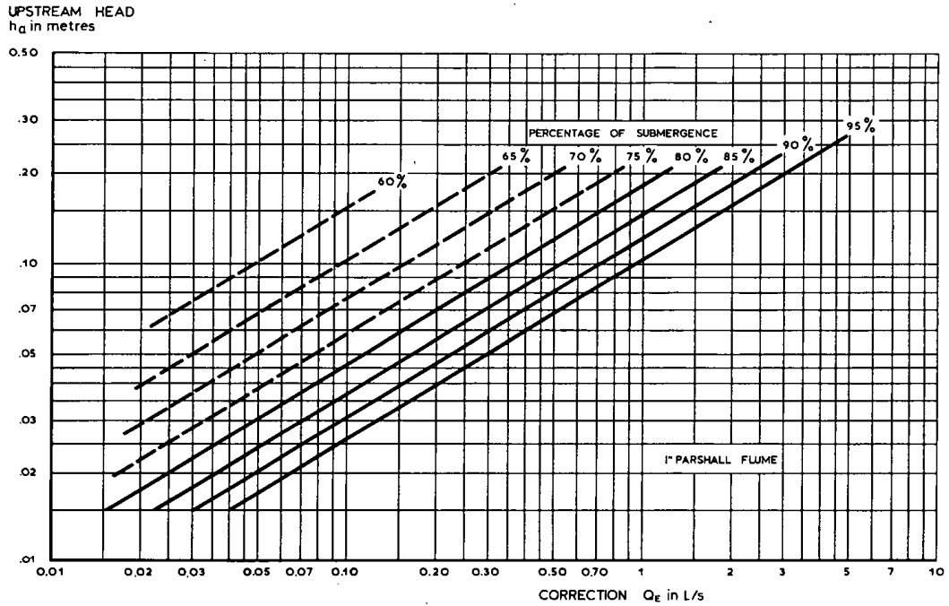
Figure 7.10 Discharge correction for submerged flow; 1" Parshall flume
