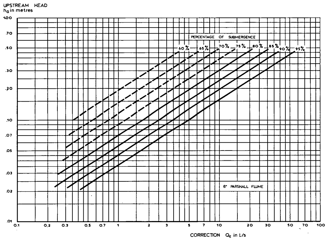
Figure 7.13 Discharge correction for submerged flow; 6" Parshall flume
