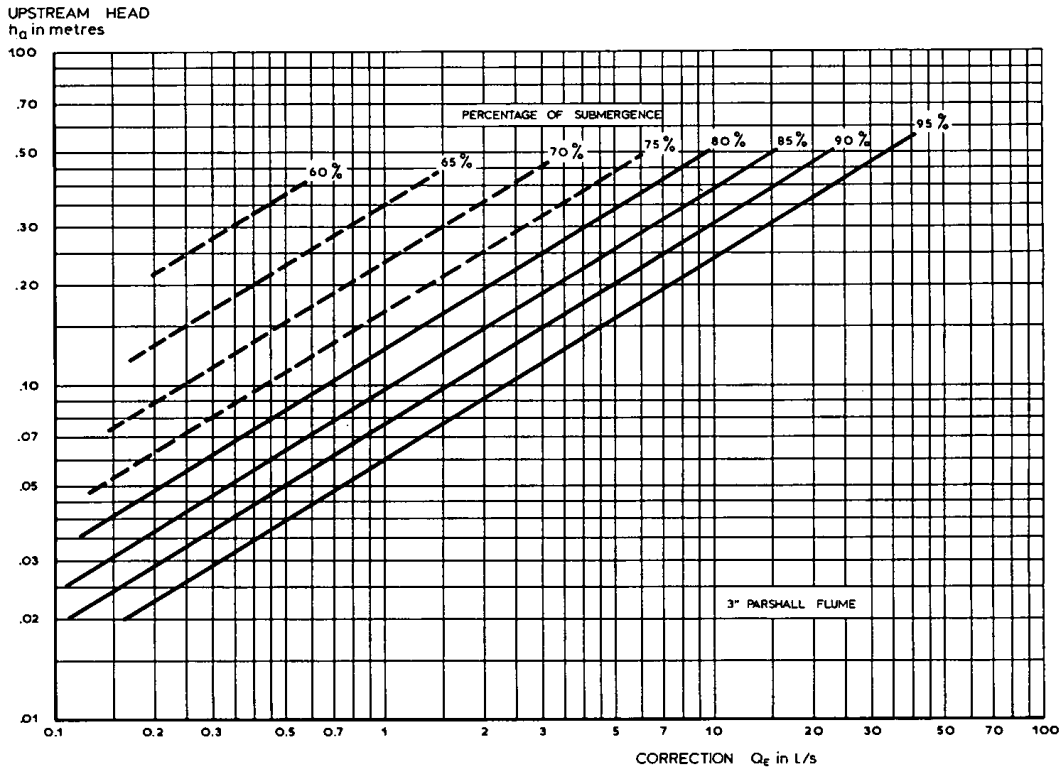
Figure 7.12 Discharge correction for submerged flow; 3" Parshall flume
