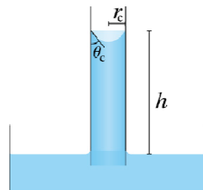
Capillary rise
