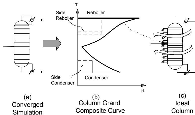
Figure 17: Procedure for obtaining Column Grand Composite Curve
