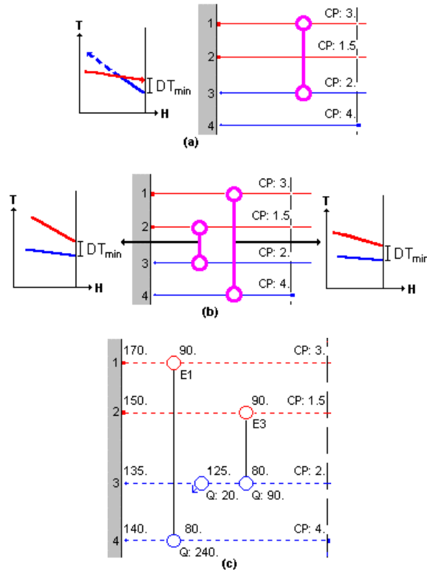
Figure 27: Criteria for temperature feasibility at the pinch
