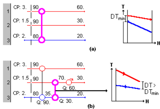
Figure 28: Network design below the pinch
