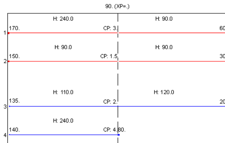
Figure 26: Grid diagram for the example problem
