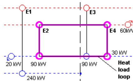
Figure 33: A heat load loop
