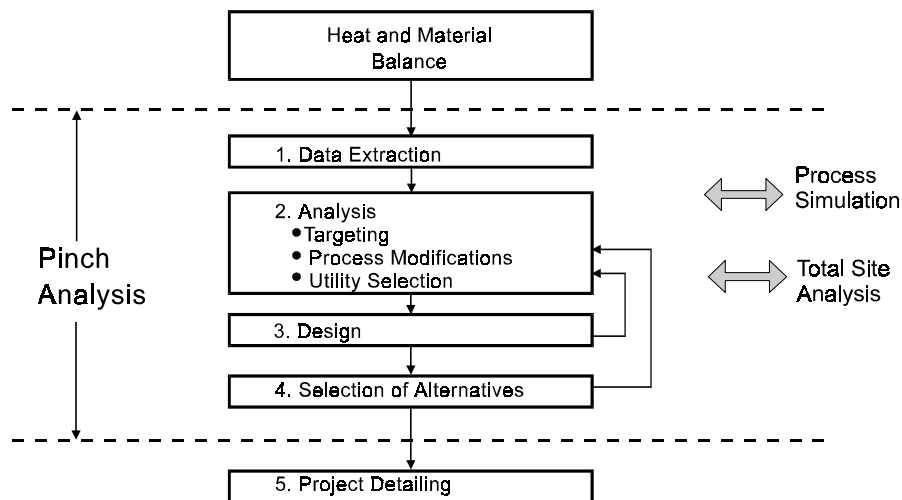
Figure 24: Key steps in Pinch Technology
