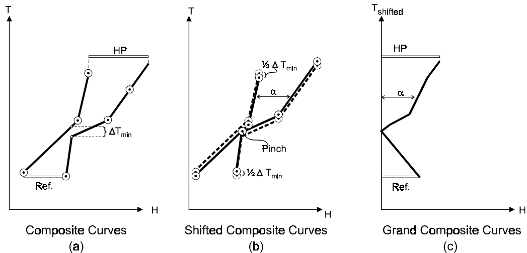
Figure 7: Construction of the Grand Composite Curve
