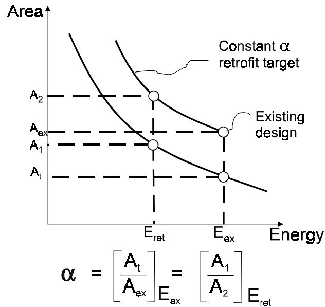
Figure 12: Area Efficiency concept
