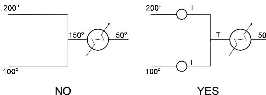
Figure 55: Isothermal mixing avoids cross-pinch heat transfer so do not mix at different temperatures.
