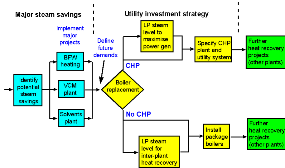
Figure 65: Total Site Road Map
