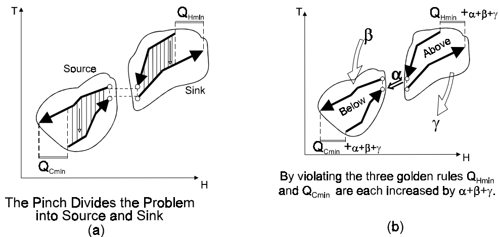
Figure 5: The Pinch Principle
