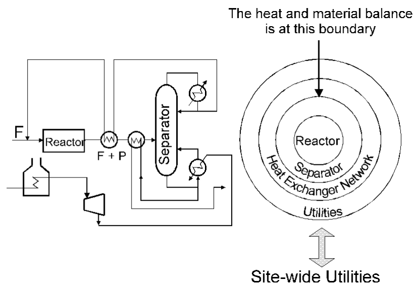
Figure 1: "Onion Diagram" of hierarchy in process design
