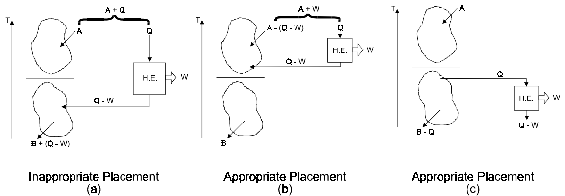
Figure 20: Appropriate Placement Principle for heat engines
