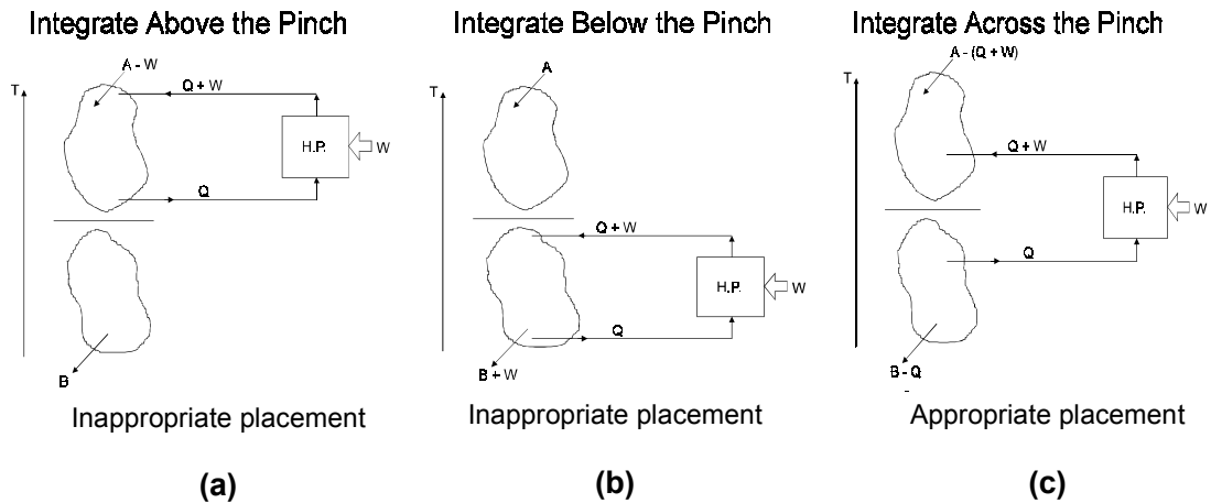
Figure 22: Placement of heat pumps.
