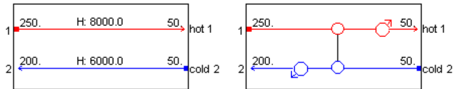
Figure 53: Improved Data Extraction and Design
