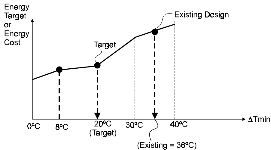
Figure 14: Targeting for retrofit applications
