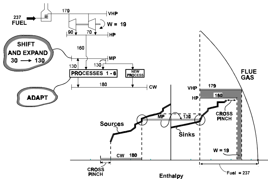
Figure 64: Alternative option based on Total Site Profiles
