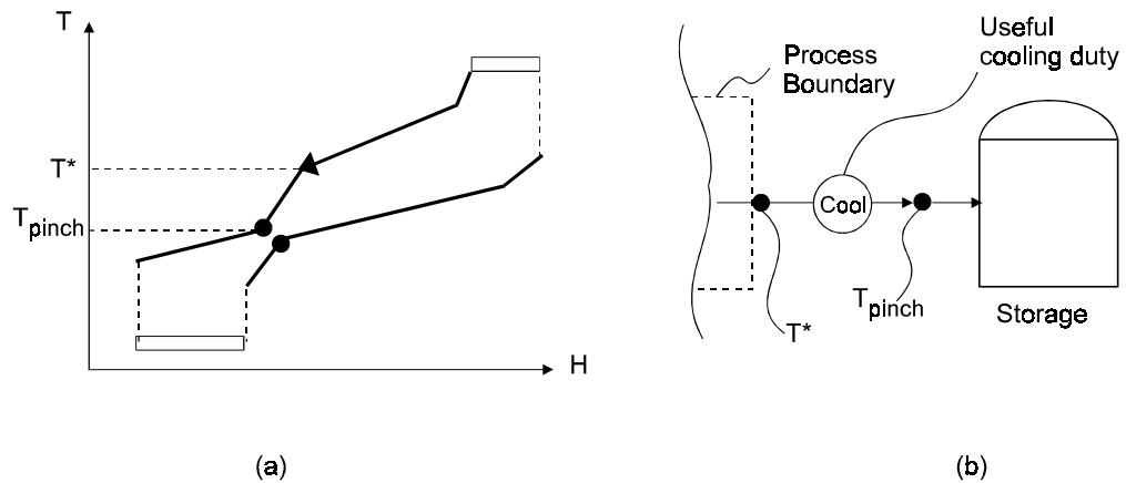
Figure 58: Stream data extraction for “soft data”.
