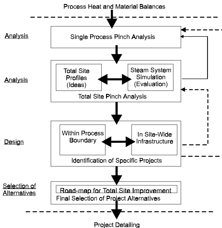
Figure 66: Key steps in total site improvement
