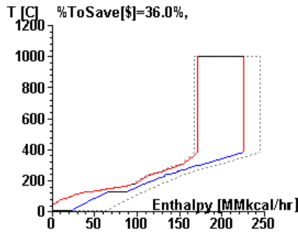
Figure 44: Example requiring Path Analysis for retrofit design
