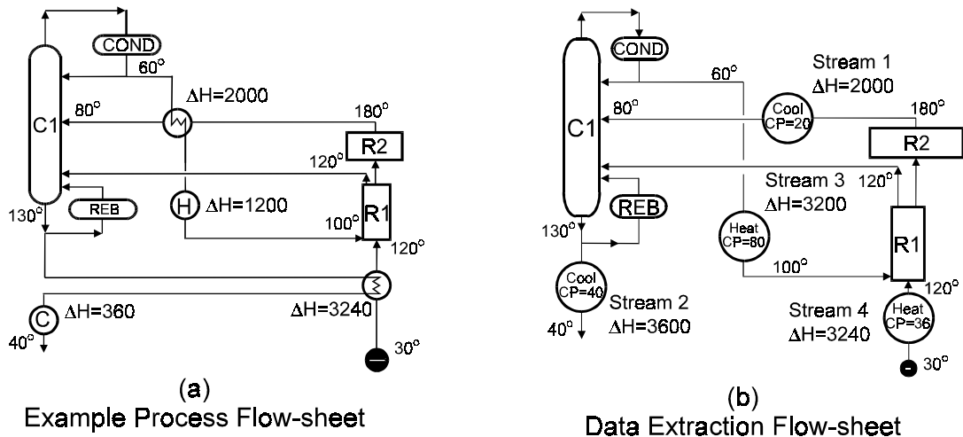
Figure 2: Data Extraction for Pinch Analysis
