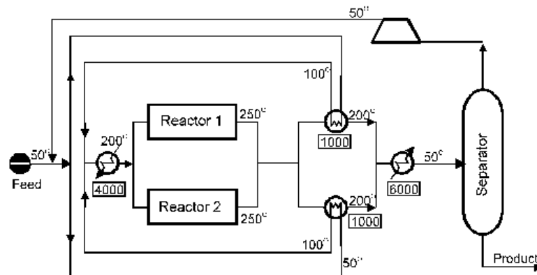
Figure 51: Example Process Flowsheet
