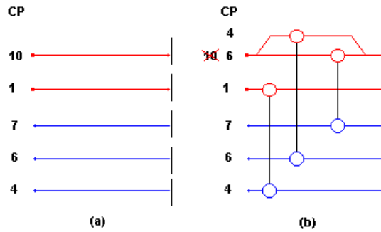
Figure 31: Incoming stream split to comply with CP_{out} \geq CP_{in} rule.
