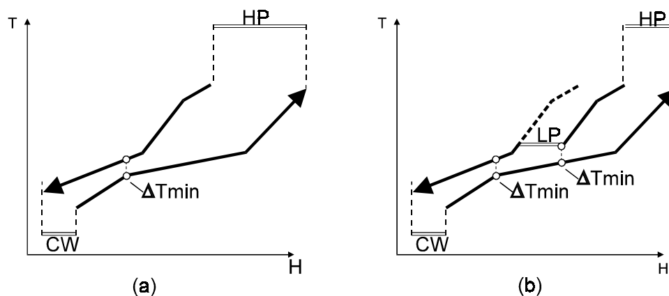
Figure 6: Using Composite Curves for Multiple Utilities Targeting
