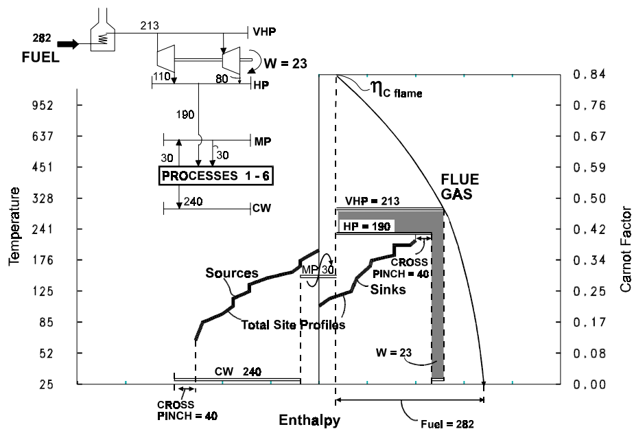
Figure 62: Existing site
