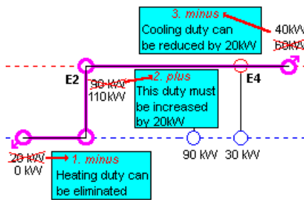
Figure 35: Using a path to reduce utility use
