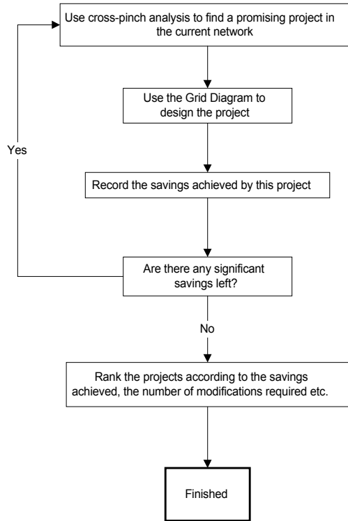
Figure 38: Procedure for correcting cross-pinch exchangers
