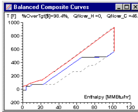
Figure 39: Example for retrofit design using Cross-Pinch Analysis
