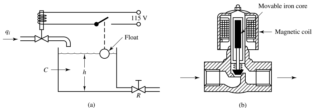
Figure 2-8 (a) Liquid-level control system; (b) electromagnetic valve.
