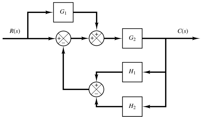
Figure 2-30 Block diagram of a system.
