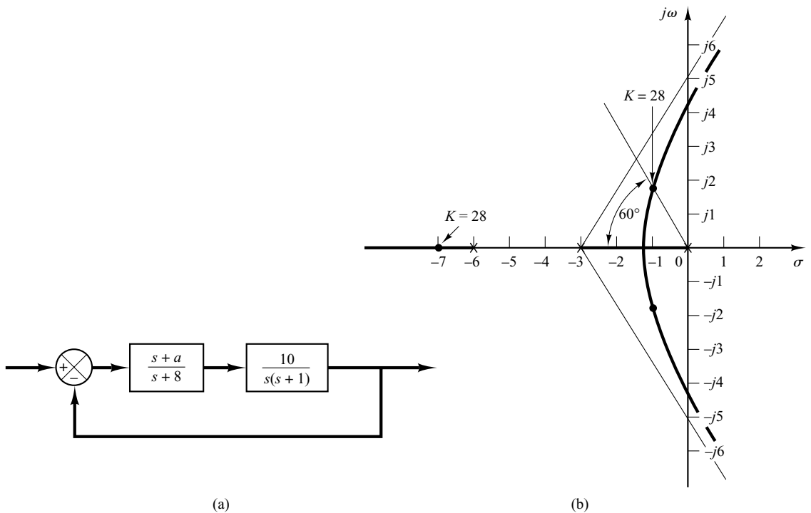
Figure 6-98 (a) Control system; (b) root-locus plot, where K = 10a .
