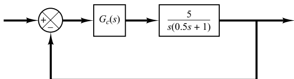
Figure 6-107 Control system.
