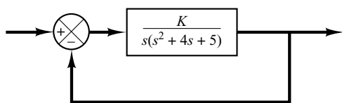
Figure 6-104 Control system.
